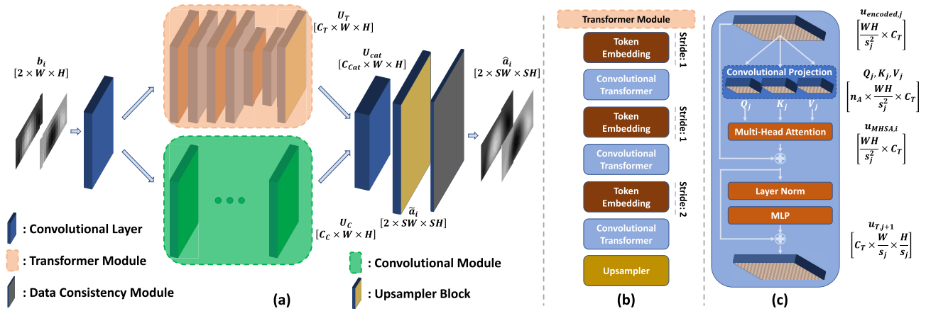
Fig. 2. (a) Schematic of the network architecture in TranSMS. After an initial convolutional layer, encoded feature maps are fed to parallel transformer and convolutional modules. The transformer module extracts contextual representations over longer distances, while the convolutional module captures localized representations. Contextual and localized feature maps are fused and upsampled to the resolution of the HR SM. Finally, a data-consistency module enforces fidelity of recovered HR SM to input LR SM. (b) The transformer module contains a cascade of token-embedding and convolutional transformer sub-blocks, and a final upsampler to restore dimensionality. (c) The transformer performs convolutional token projection, followed by MHA and MLP blocks to extract contextual features.
