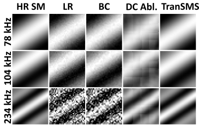
Fig. 8. A pre-trained TranSMS model was used to super-resolve a 64 \times 64 HR SM by processing overlapping 16 \times 16 patches in the input 32 \times 32 LR SM. SM rows for different harmonics at 45^\circ are shown. Recovered HR SMs are shown under 30 dB measurement SNR, along with the input LR SM and the reference HR SM.
