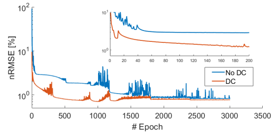
Fig. 4. Validation performance of TransSMS with (red curve) and without (blue curve) the data-consistency (DC) module. The HR SM recovery performance is reported as nRMSE across training epochs. The upper-right panel displays a zoomed-in portion of nRMSE curves during the initial stages of training.
