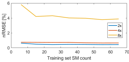
Fig. 5. SM recovery performance of TranSMS as a function of the number of SMs included in the training set for SR factors of 2\times - 8\times .
