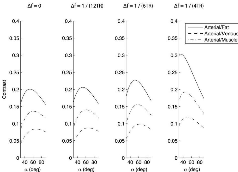
FIG. 4. The warping of synthesized profiles at different \Delta f values has an effect on signal contrast. An analysis of arterial/venous, arterial/muscle, and arterial/fat contrast is shown above as a function of both flip angle and resonant shift \Delta f . As in Figure 3, graphs are shown for \Delta f = 0, 1/(12TR), 1/(6TR) , and 1/(4TR) . Interestingly, the distortion tends to improve the contrast of the relevant tissues for the peripheral angiography application.
