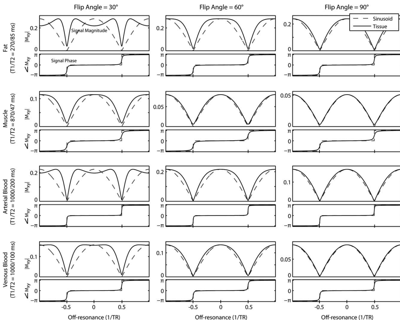
FIG. 1. The bSSFP signal as a function of off-resonance (solid line) is compared with a sinusoid (dashed line) for several tissues (fat, muscle, arterial blood, and venous blood) at flip angles of 30°, 60°, and 90°. As flip angle is increased, the bSSFP signal begins to more closely approximate a sinusoid for many tissues.
